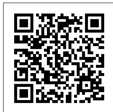
Example Problem of Enthalpy Change of a Reaction
